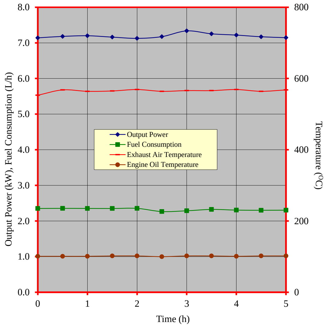
Figure 3. Performance characteristic curves during the continuous running test of the SUMO SM120P Diesel engine
