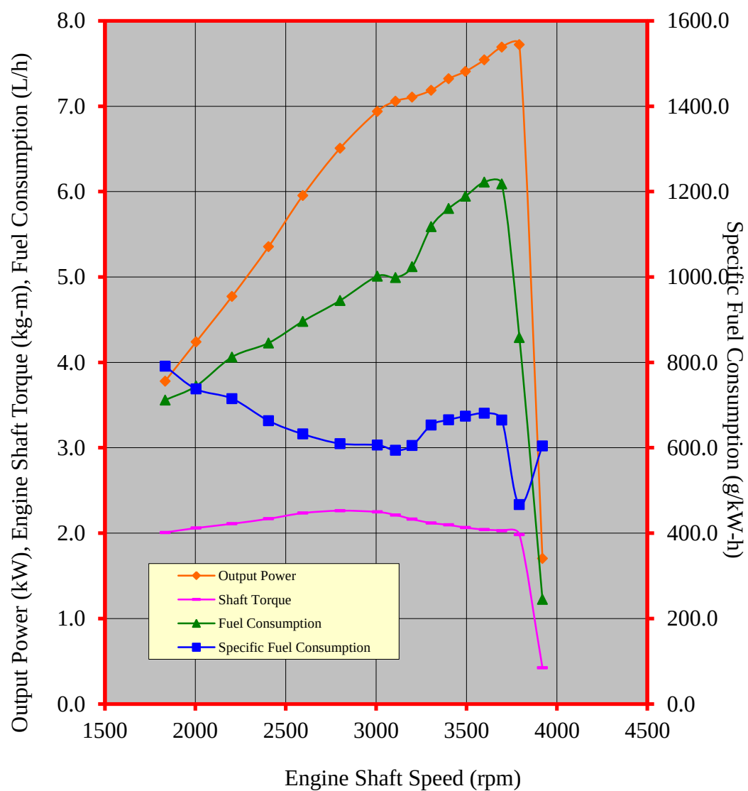
Figure 2. Performance characteristic curves of the SUMO SM120P Diesel engine
